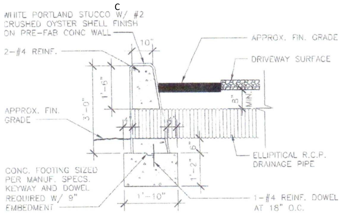
2 TYP. CULVERT HEADWALL SECT. PRE-CAST WALL SCALE: 1/2"=1'-0"
