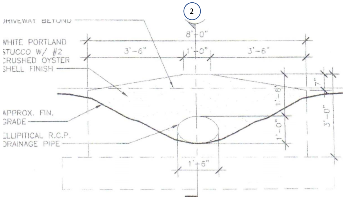
1 TYP. CULVERT HEADWALL ELEV. PRE-CAST WALL SCALE: 1/2"=1'-0"
